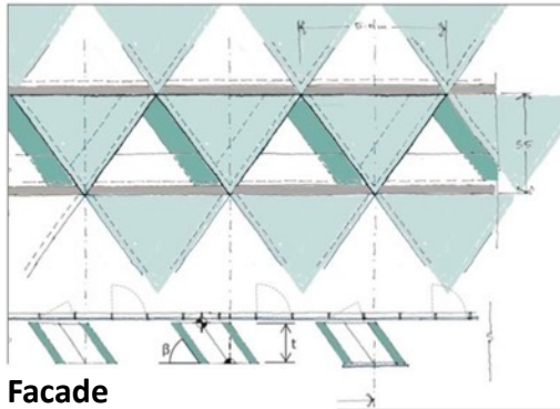
V-Supports
